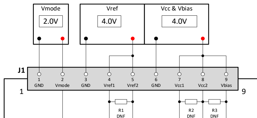
Figure 57 – EV90A006 Standard Power Supply Connections
