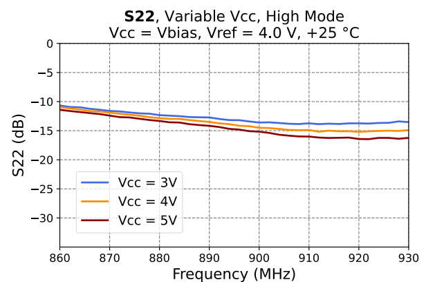
Figure 13 - Output Return Loss vs. Vcc
