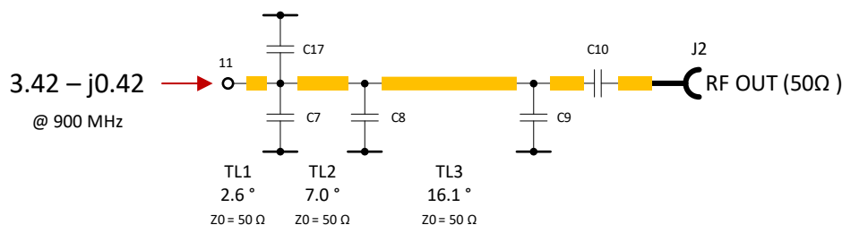
Figure 54 – Diagram of the EV90A006 Output Matching Network
