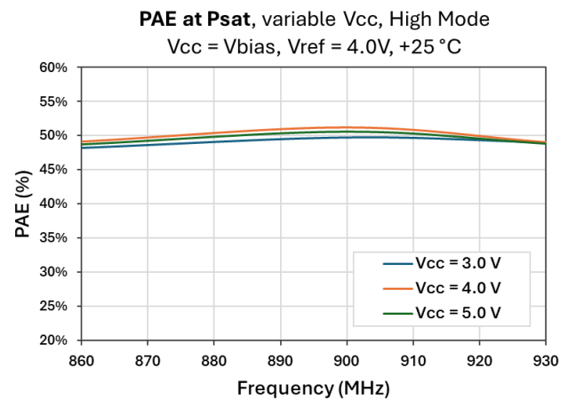
Figure 29 - PAE at Psat
