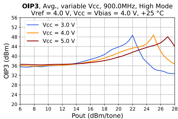
Figure 46 - OIP3 vs. Pout at 900 MHz
