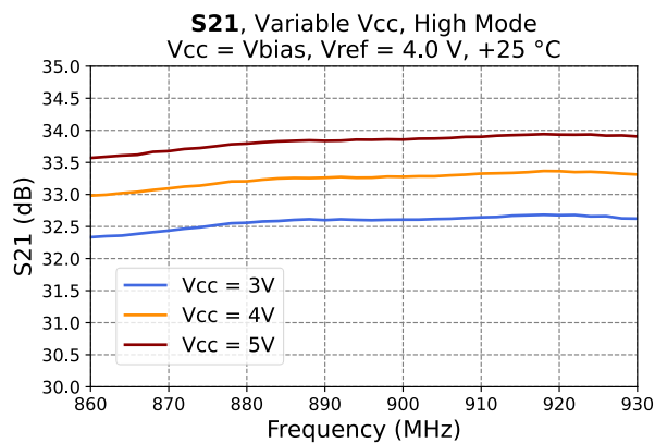
Figure 10 - Small Signal Gain vs. Vcc
