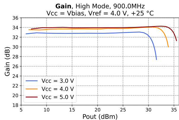
Figure 17 - Gain vs. Output Power at 900 MHz
