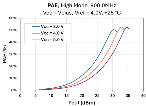
Figure 22 - PAE vs. Output Power at 900 MHz
