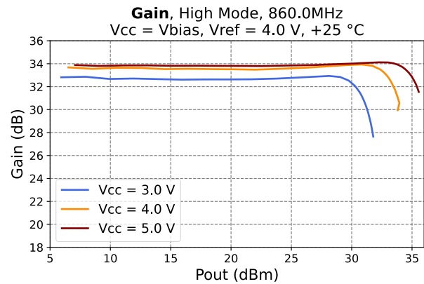
Figure 15 - Gain vs. Output Power at 860 MHz
