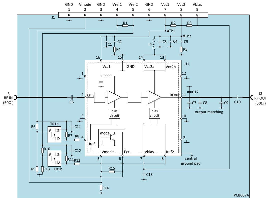
Figure 51 - EV90A006 Schematic
