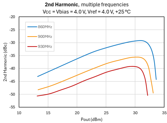
Figure 49 - Second Harmonic vs. Pout
