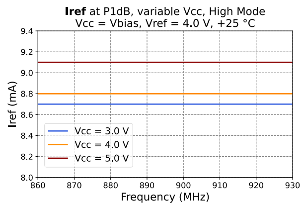
Figure 41 - I_{ref} at P1dB
