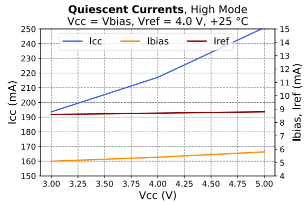
Figure 39 - Idle Currents vs. Vcc
