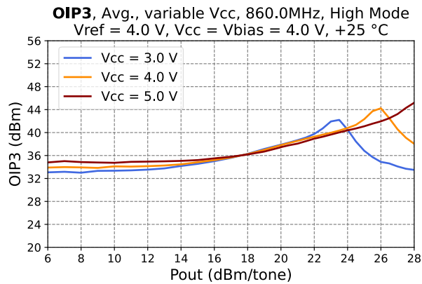
Figure 44 - OIP3 vs. Pout at 860 MHz
