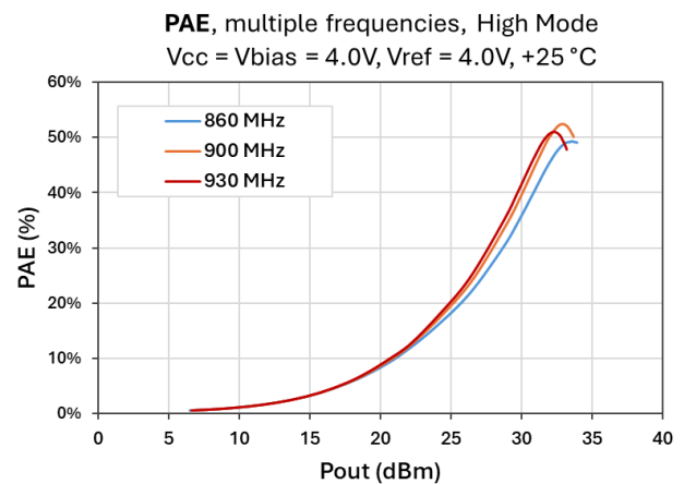
Figure 25 - PAE vs. Output Power
