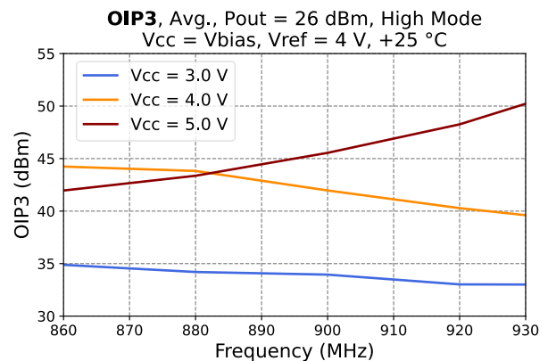
Figure 47 - OIP3 vs. Frequency at Pout = 26 dBm/ton
