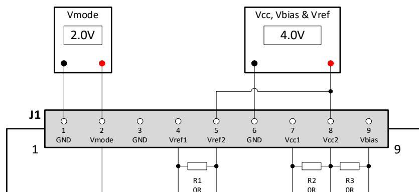
Figure 58 - Alternative EV90A006 Power Supply Connections with R1, R2 and R3 fitted
