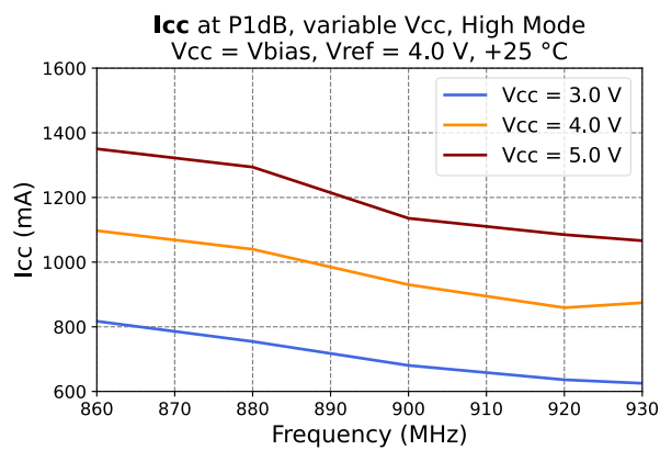
Figure 40 - I_{cc} at P1dB
