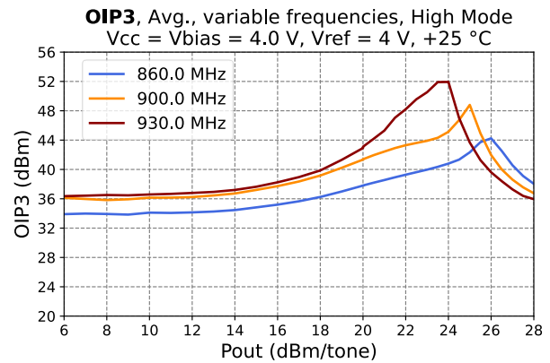
Figure 45 - OIP3 vs. Pout
