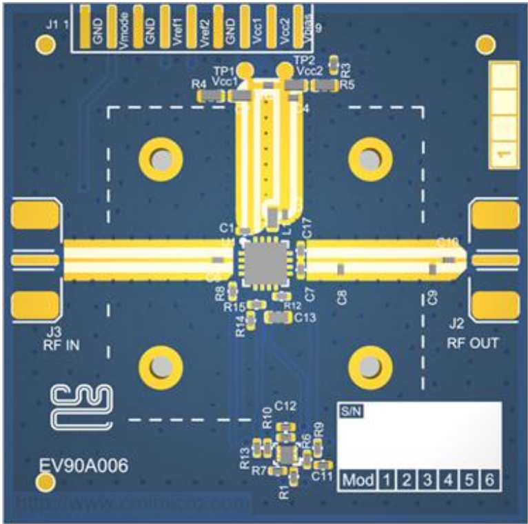
Figure 53 - EV90A006 PCB Top Layer View
