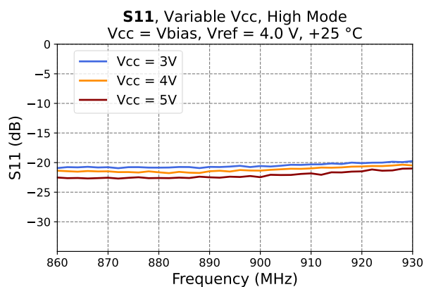
Figure 12 - Input Return Loss vs. Vcc
