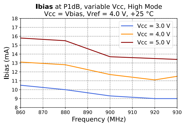
Figure 42 - I_{bias} at P1dB
