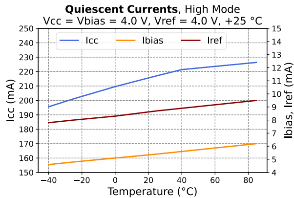
Figure 38 - Idle Currents vs. Temp
