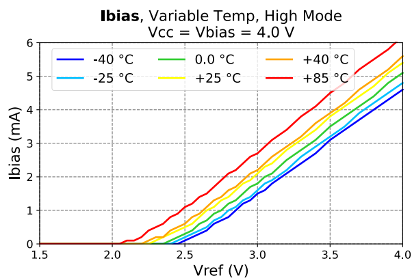
Figure 36 - I bias vs. V ref over Temp
