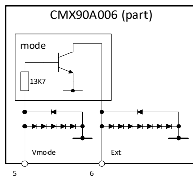
Figure 55 – Vmode Pin Internal Configuration
