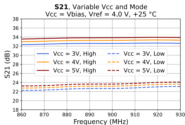
Figure 7 - Small Signal Gain (Low and High Modes)
