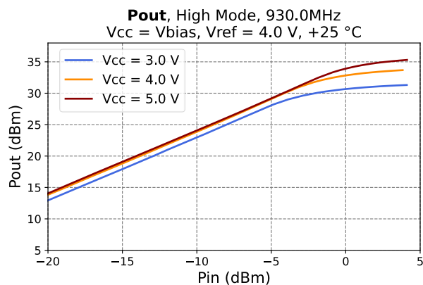
Figure 18 - Output Power vs. Input Power at 930 MHz
