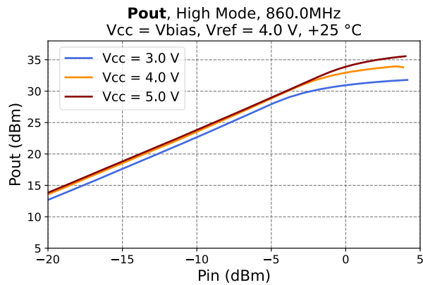
Figure 14 - Output Power vs. Input Power at 860 MHz
