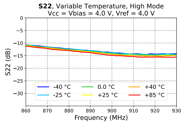
Figure 9 - Output Return Loss (S22)
