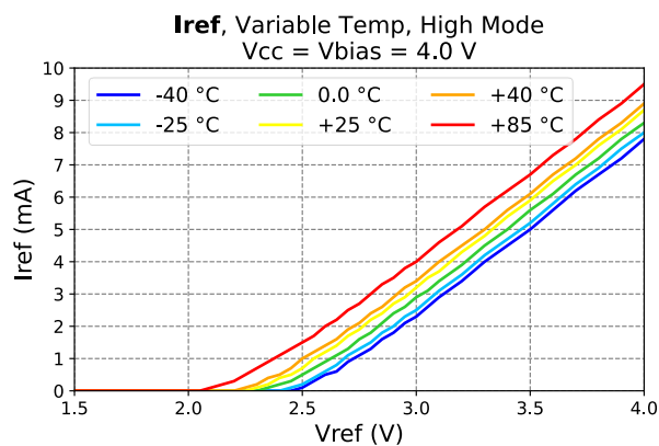
Figure 34 - I ref vs. V ref over Temp
