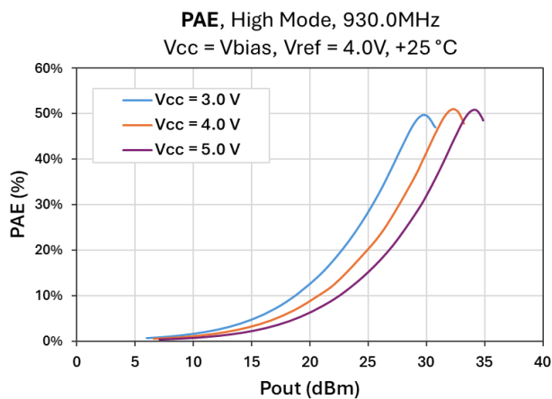
Figure 24 - PAE vs. Output Power at 930 MHz
