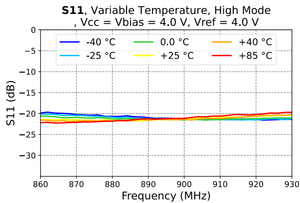
Figure 8 - Input Return Loss (S11)
