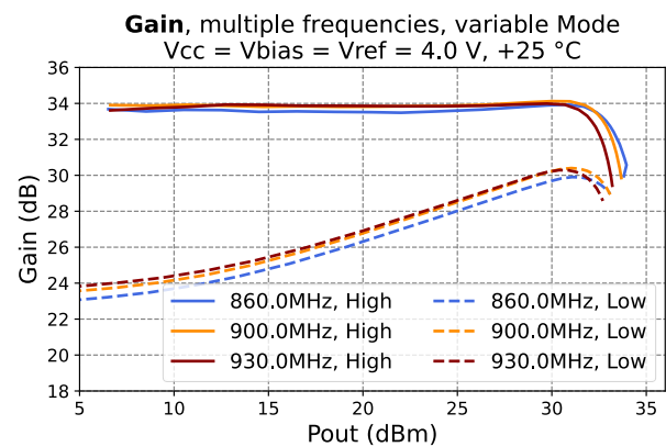
Figure 31 - Gain vs. Pout (Low and High Modes)
