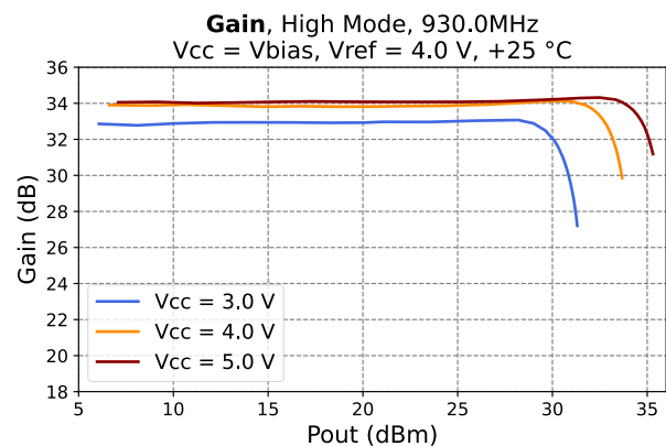
Figure 19 - Gain vs. Output Power at 930 MHz
