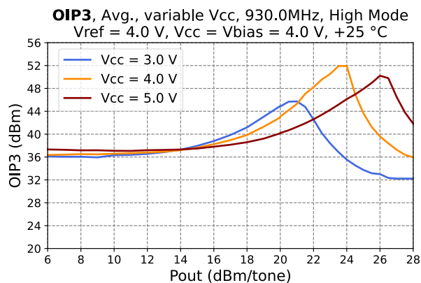
Figure 48 - OIP3 vs. Pout at 930 MHz
