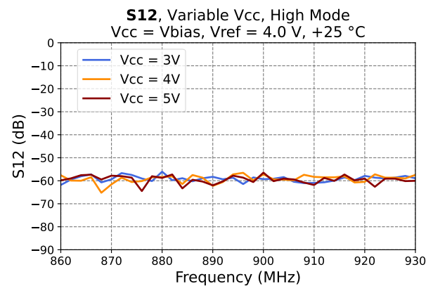
Figure 11 - Reverse Isolation vs. Vcc
