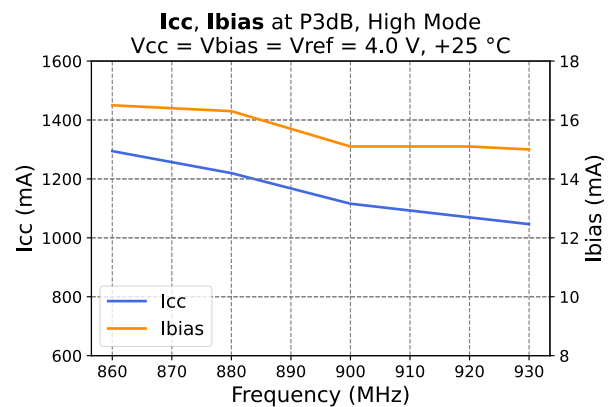
Figure 43 - I_{cc} and I_{bias} at P3dB
