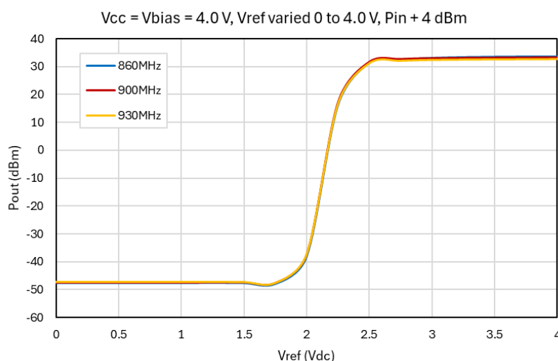
Figure 56 - Vref Power Control
