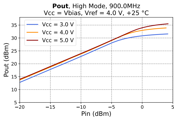
Figure 16 - Output Power vs. Input Power at 900 MHz
