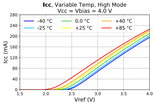
Figure 32 - I cc vs. V ref over Temp
