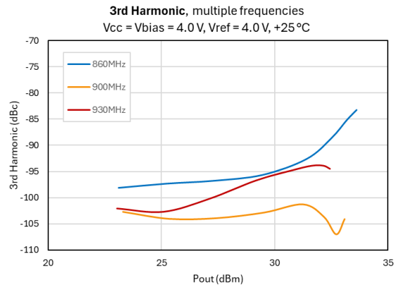
Figure 50 - Third Harmonic vs. Pout
