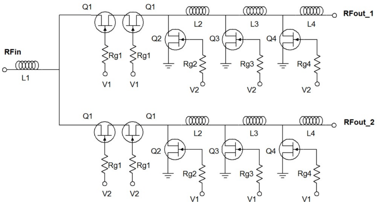
Schematic of the SPDT GaN switch
