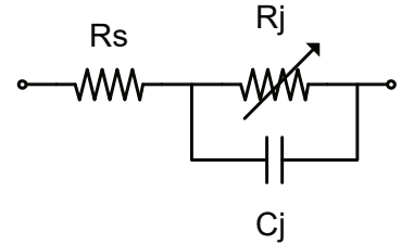
Electrical equivalent model of a PIN diode
