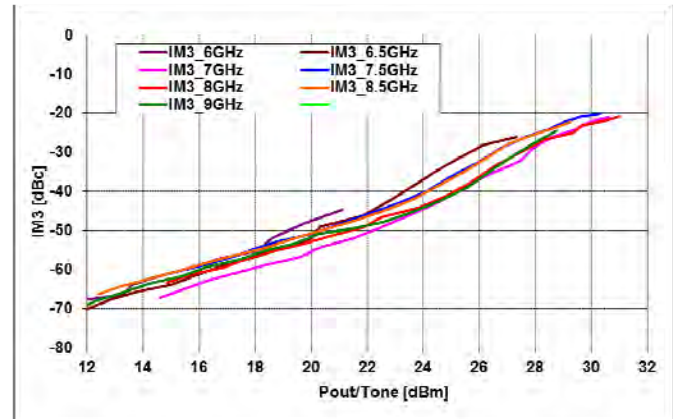
IM3 Level [dBc] vs. output power/tone [dBm]
