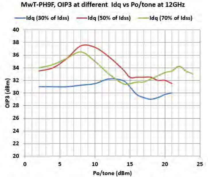
MwT-PH9F, Load Pull data for Power, Vds=8V, Idq=0.7xIdss
