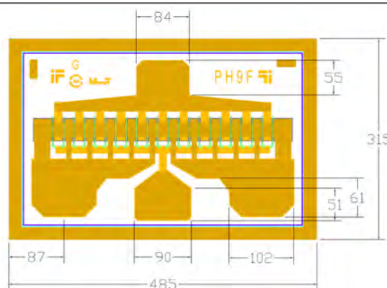
Chip Dimensions: 485 x 315 \mu\text{m} Chip Thickness: 100 \mu\text{m}
