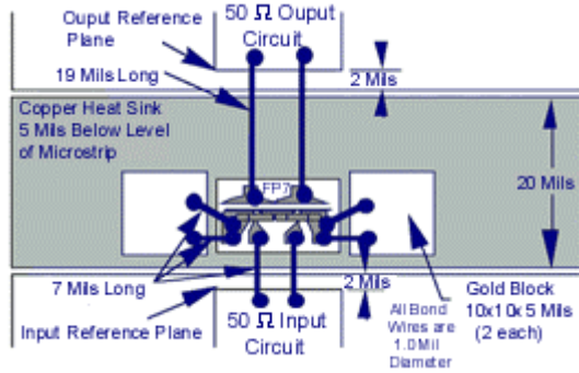
MwT-PH7F DUAL BIAS
