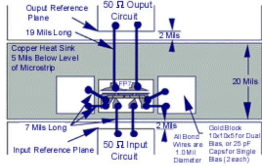
MwT-PH7F SELF BIAS
