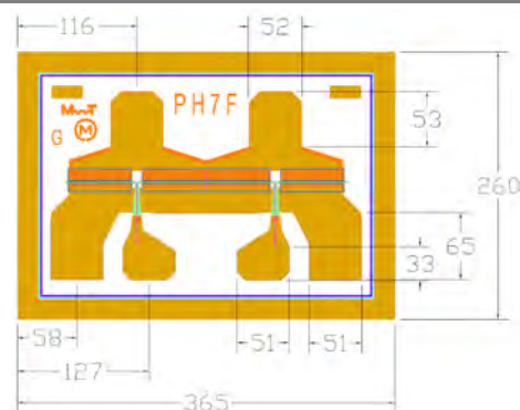
Chip Dimensions: 365 x 260 microns Chip Thickness: 100 microns
