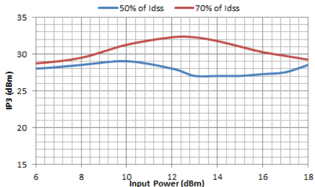
MwT-PH7F, OIP3 vs Po/1tone with different Idq (% of Idss)
