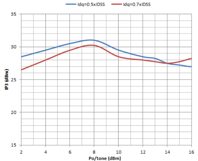
MwT-PH33F, Load Pull Data, Vdq=8V; Idq=0.7xIdss
