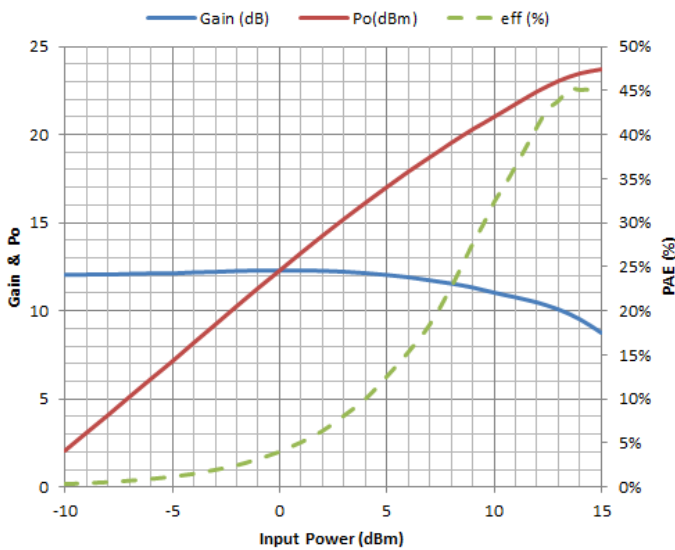
MwT-PH33F, Load Pull Data, Vdq=8V; Idq=0.7xIdss
