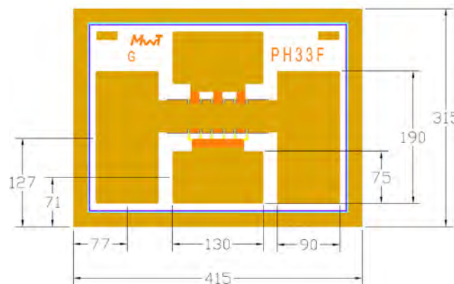
Chip Dimensions: 415 x 315 microns Chip Thickness: 100 microns
