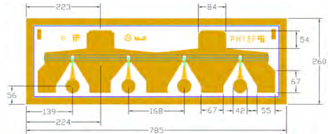
Chip Dimensions: 785 x 260 \mu\text{m} Chip Thickness: 100 \mu\text{m}
