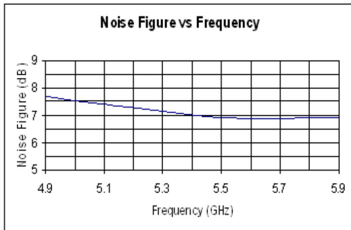
Figure 8 Noise Figure
