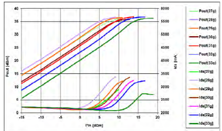
Po (dBm), and Ids (mA) vs. Pin (dBm)
