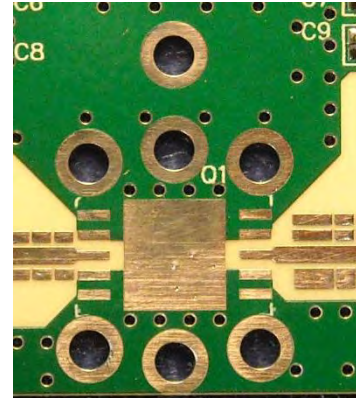
Figure 4 Hole Pattern
