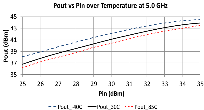
Figure 4 Pout vs Pin over Temperature
