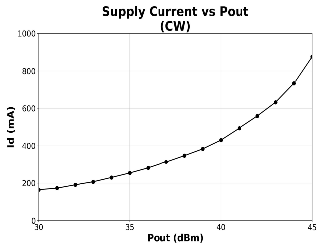
Figure 3 Supply Current
