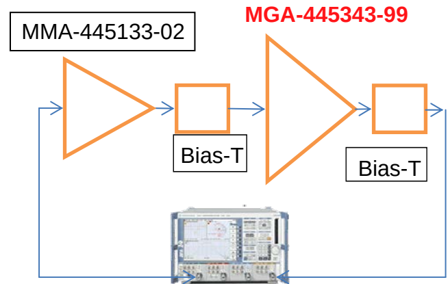
Figure 1 Test Setup
