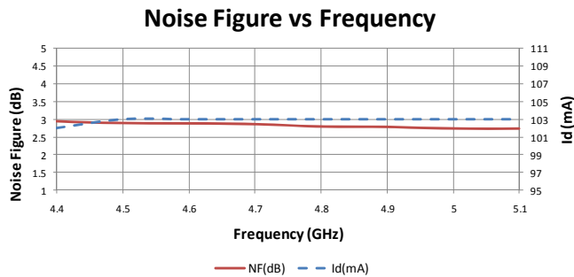
Figure 2 Noise Figure
