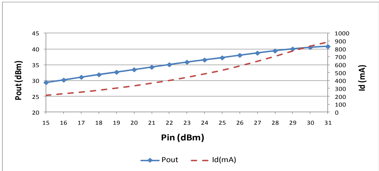
Figure 5 Pout vs Pin Using Constant Current Loop
