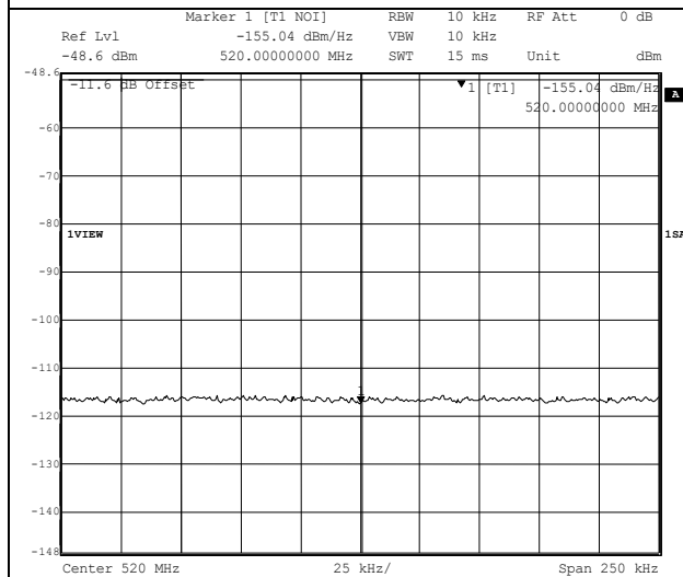
500 MHz noise floor, carrier at 500 MHz
