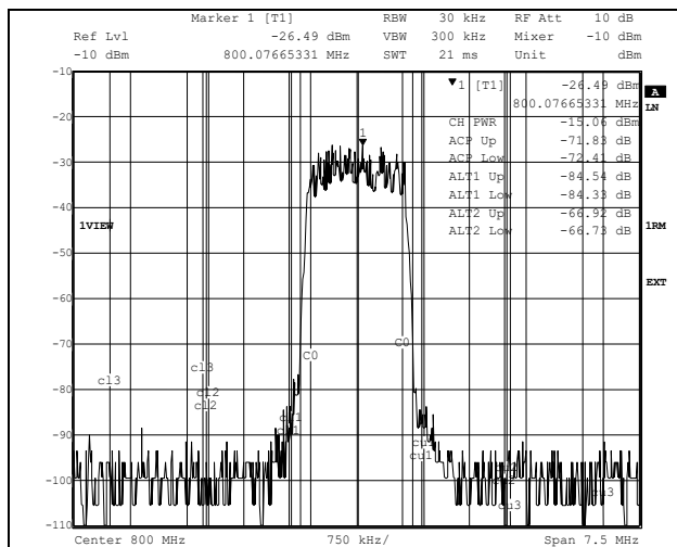
IS-95 reverse channel operation at 800 MHz, measured at 885 kHz, 1.98 kHz and 2.65 MHz
