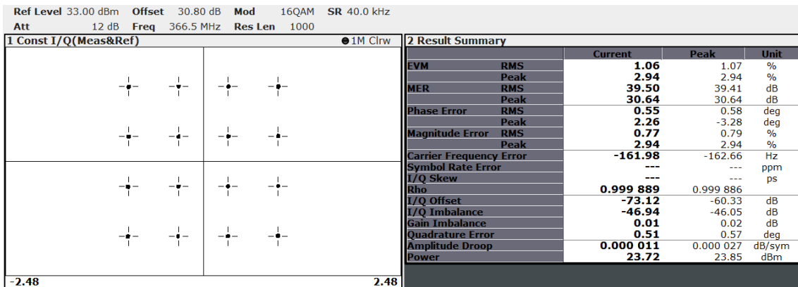
Figure 28 16-QAM, 40 ks/s, Constellation and EVM at 366.5MHz
