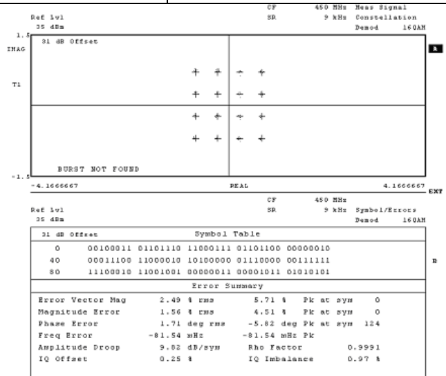
Error Vector
