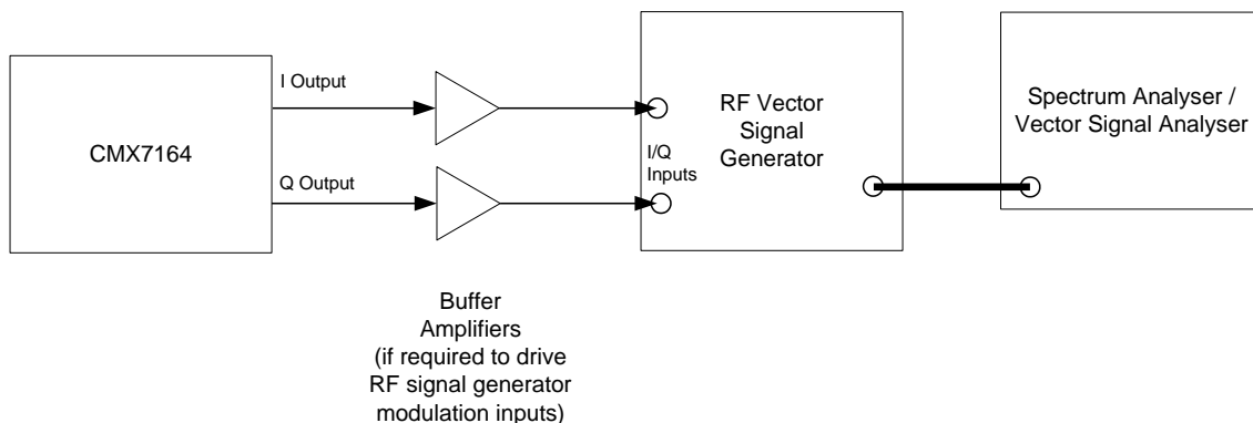
Figure 58 Tx Spectrum and Modulation Measurement Configuration for I/Q Operation
