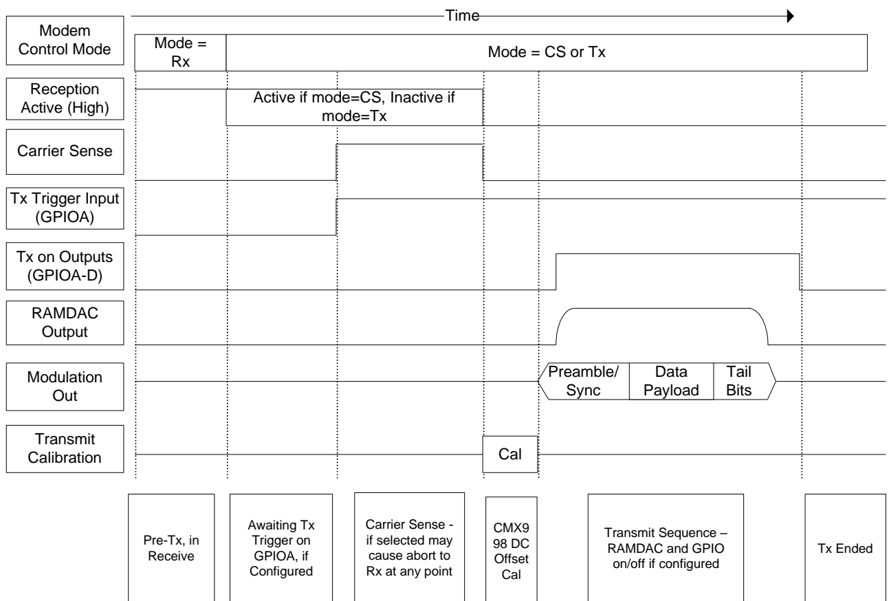
Figure 19 Transmit Sequence
