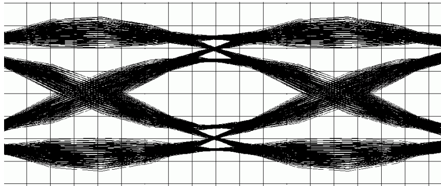
Figure 28 Received Eye Diagram7364 FI-1.x
