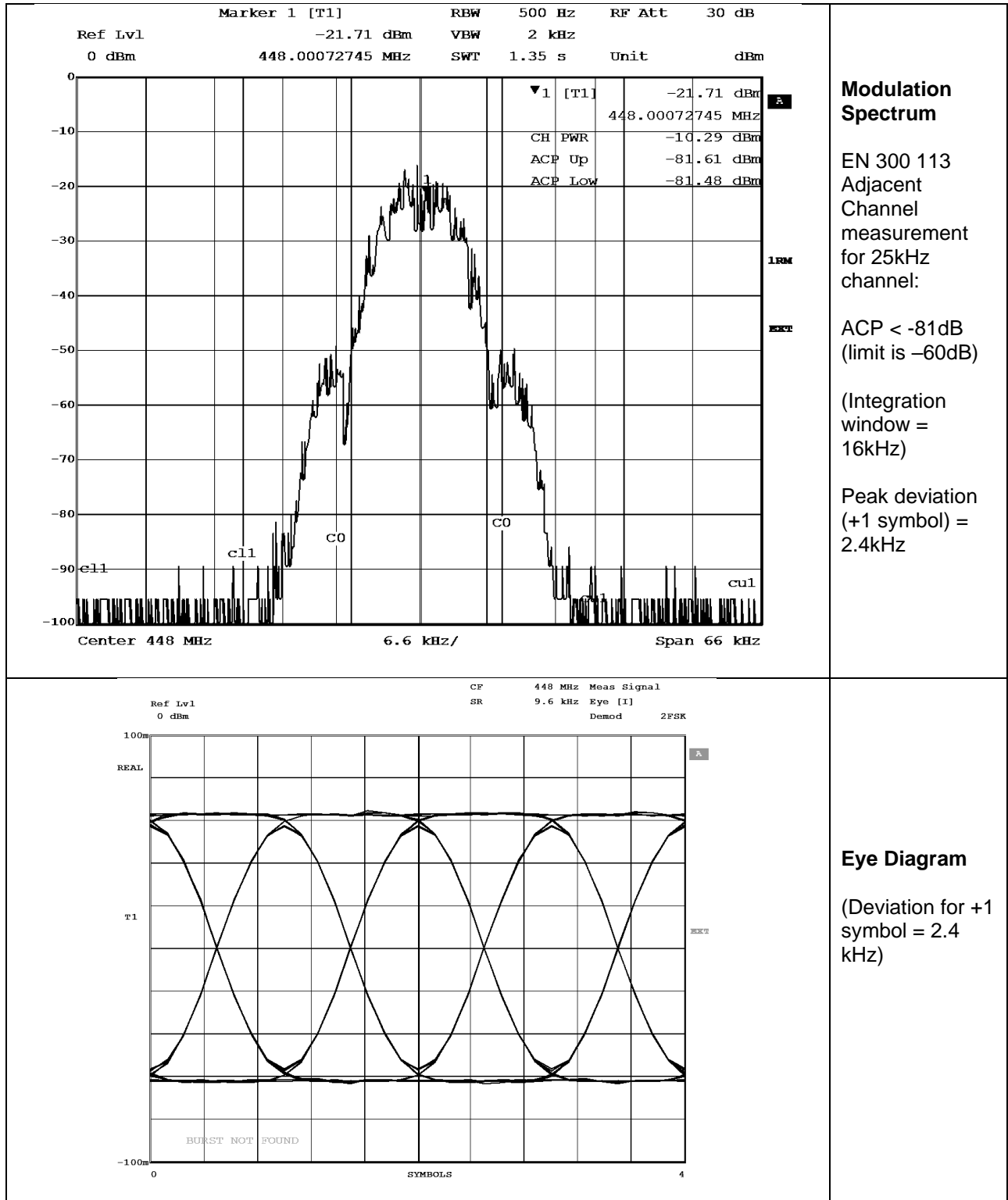
Figure 45 Tx Modulation Spectra (GMSK), 9.6kbps (BT=0.5), I/Q Modulation
