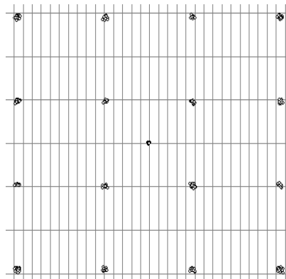
Figure 29 Sample at Symbol Timing with I/Q DC Offset Diagnostic Mode (no frequency error)
