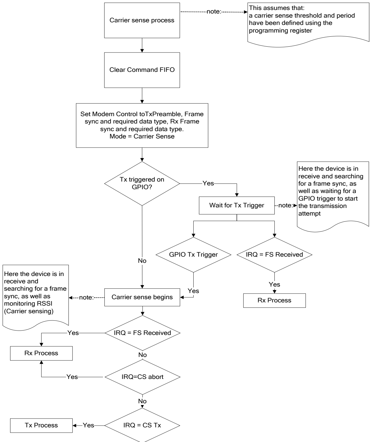
Figure 18 Carrier Sense
