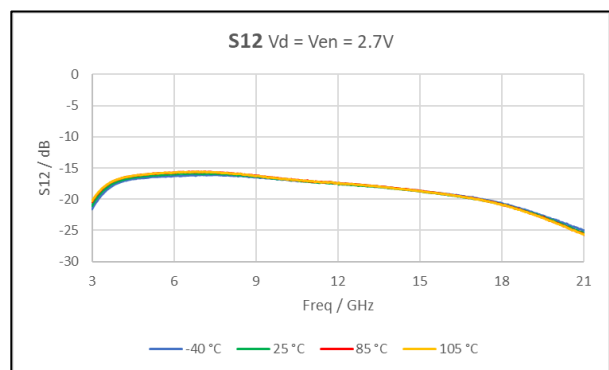
Figure 24: S12 Vd = Ven = 2.7V
